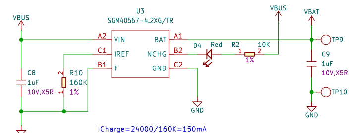
Battery charging circuit
