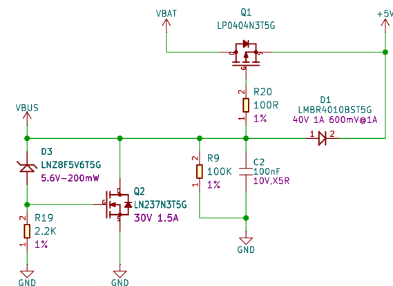
Power switching circuit
