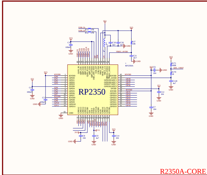
R2350A-CORE
