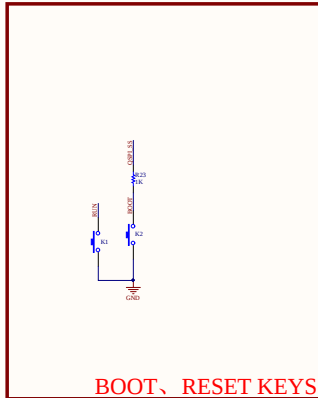
BOOT、RESET KEYS
