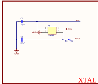
XTAL
