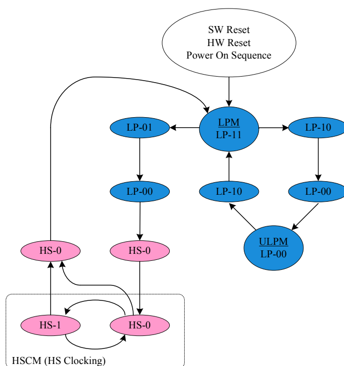
Flow chart of the different clock lanes
